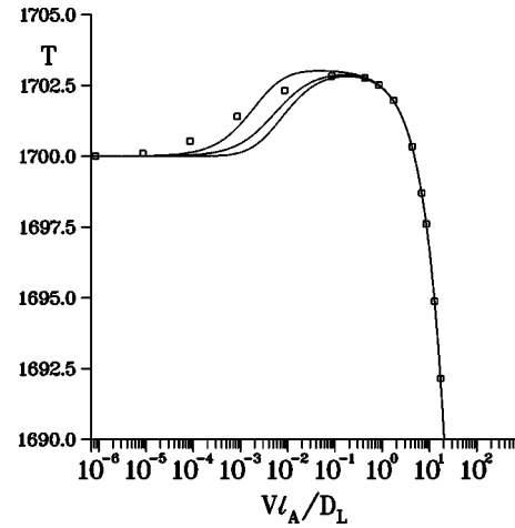
FIG. 6. Data points denote the temperature (in K) obtained from our calculations for different values of growth velocity V by using the logarithmic model (47) for D(\phi) with D_S / D_L = 10^{-5} . The upper curve shows the temperature given by Eq. (14) without solute drag ( \alpha = 0 ), the lower curve shows the temperature given by this expression with solute drag ( \alpha = 1 ), and the middle curve shows the temperature given by this expression with the asymptotic value ( \alpha = 24/35 ).
